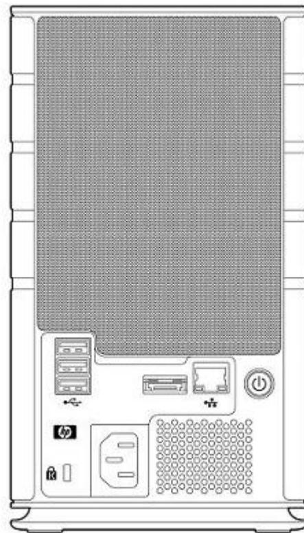
HP StorageWorks X500 Data Vault rear view
